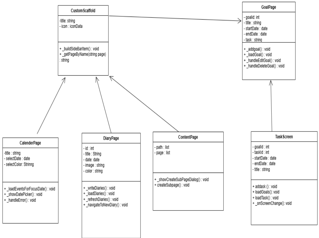
FIGURE 4: DESIGN CLASS DIAGRAM
