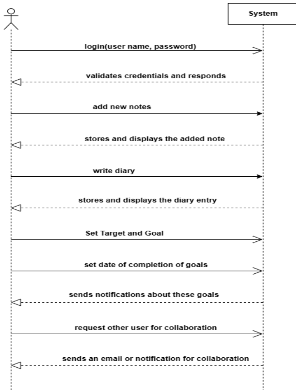
FIGURE 3: SYSTEM SEQUENCE DIAGRAM (SSD)
